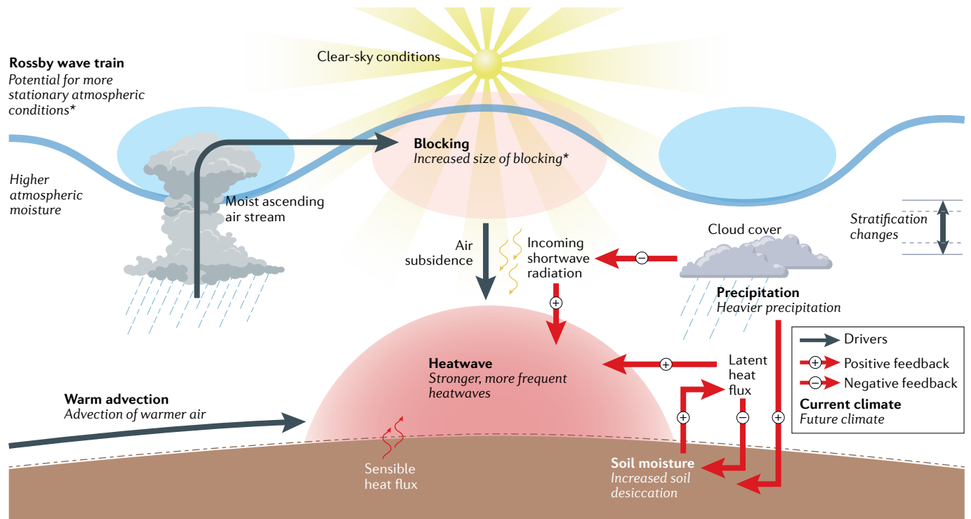
Fig. 2 | Schematic representation of processes contributing to mid-latitude summer heatwaves. Black arrows represent driving mechanisms and red arrows feedbacks, wherein + indicates a positive feedback and – a negative feedback. Boldface text indicates processes in current climate and italic text projected changes under anthropogenic warming. Asterisks indicate projected changes
